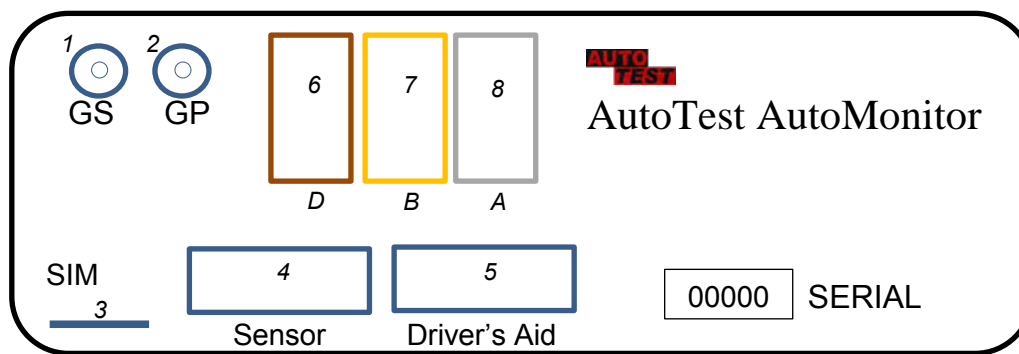
Figure 3: AutoMonitor - Rear view
